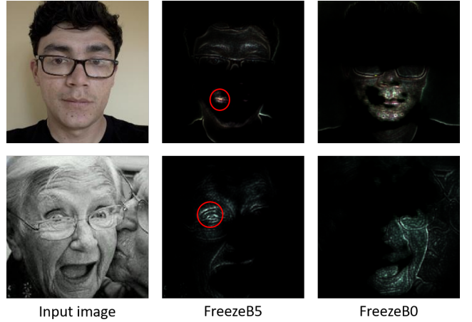
Figure 5: Visualization of the difference between the saliency maps of FreezeB5 and FreezeB0 for contempt (top) and surprise (bottom) images. The red circles highlight the areas that correlate with the action units which FreezeB5 paid more attention to.
