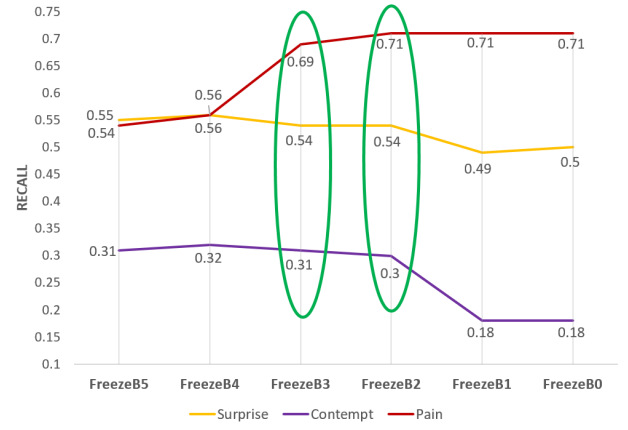
Figure 7: Plot of pain, surprise, and contempt recalls of the 6 pain models. The green ellipses highlight the best models that have a good balance between pain and emotion recalls.
