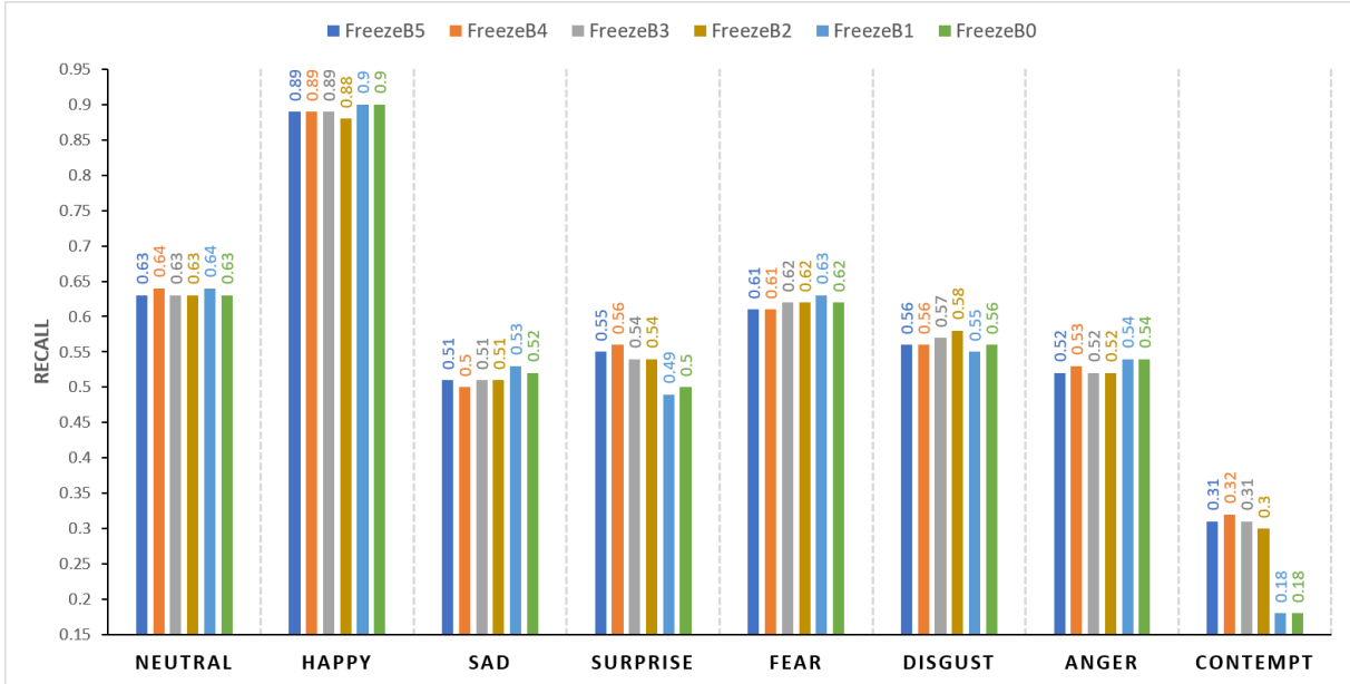
Figure 4: Class-wise recalls of the six pain models obtained by re-training their output layers for emotion recognition.
