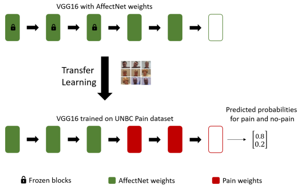
Figure 1: Illustration of the process we followed for transfer learning from emotion to pain. This images shows the process of generating the model FreezeB3 by freezing the first 3 blocks of the emotion model.
