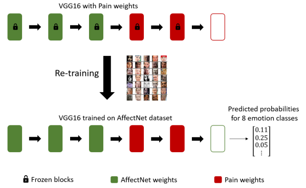
Figure 2: Illustration of the process we followed for re-training the various pain models. All convolution blocks are frozen and only the output layers are trained to predict emotions instead of pain.
