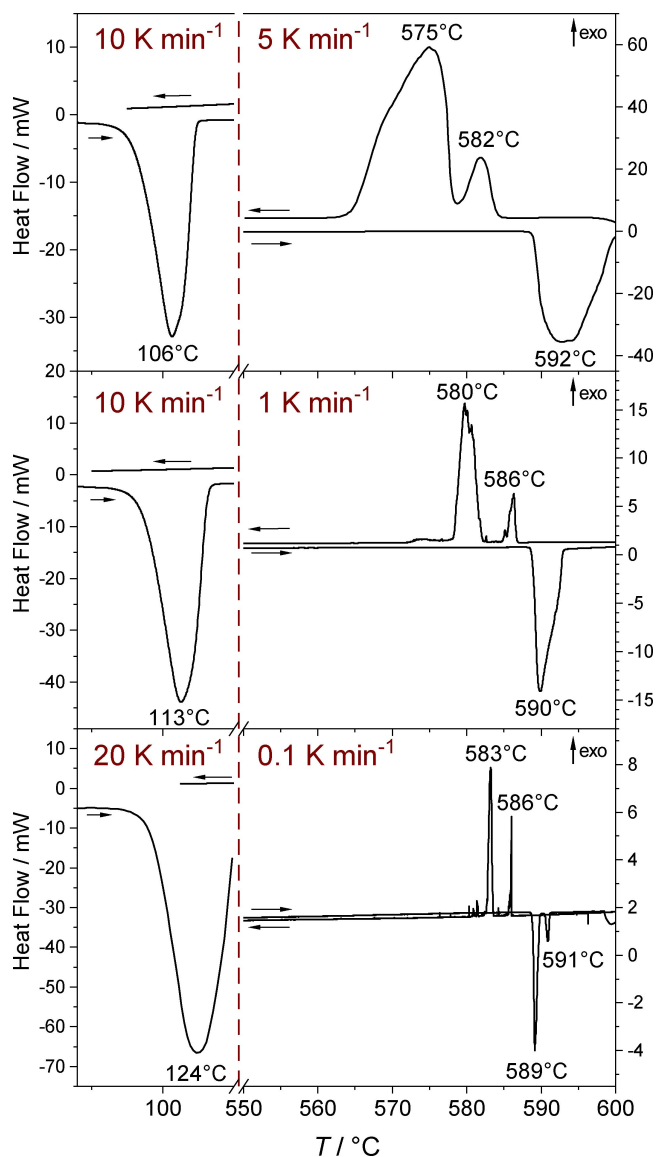
Figure 1. DSC signals of \text{Na}_2\text{WO}_4 \cdot 2\text{H}_2\text{O} for various heating and cooling rates; the endothermic event upon heating around 590 °C is split into two peaks at a slow heating rate of 0.1 \text{K min}^{-1} .
