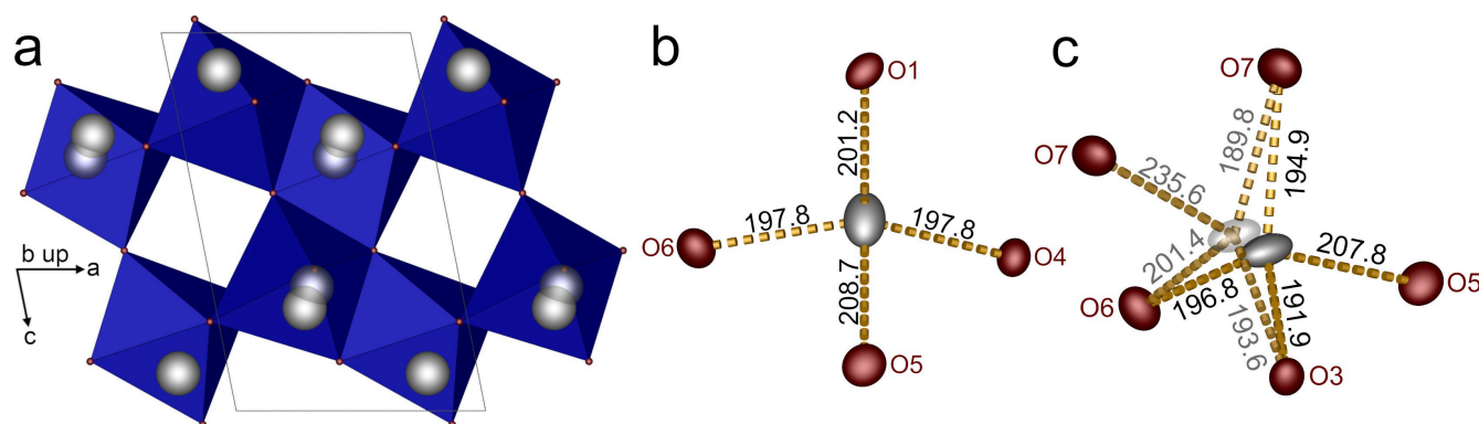
Figure 6. (a) Unit cell of \text{Li}_2\text{W}_2\text{O}_7 along (010): tungstate octahedra are shown in blue, oxygen atoms in red and lithium atoms in grey; for the latter, the minority variant is shown semitransparent; (b) \text{Li}1\text{O}_4 tetrahedron; (c) disorder of the Li2 site: the minority variant (Li2B) is shown semitransparent, the majority variant (Li2A) opaque; the Li–O distances are given in pm; ellipsoids are shown at 80% probability.
