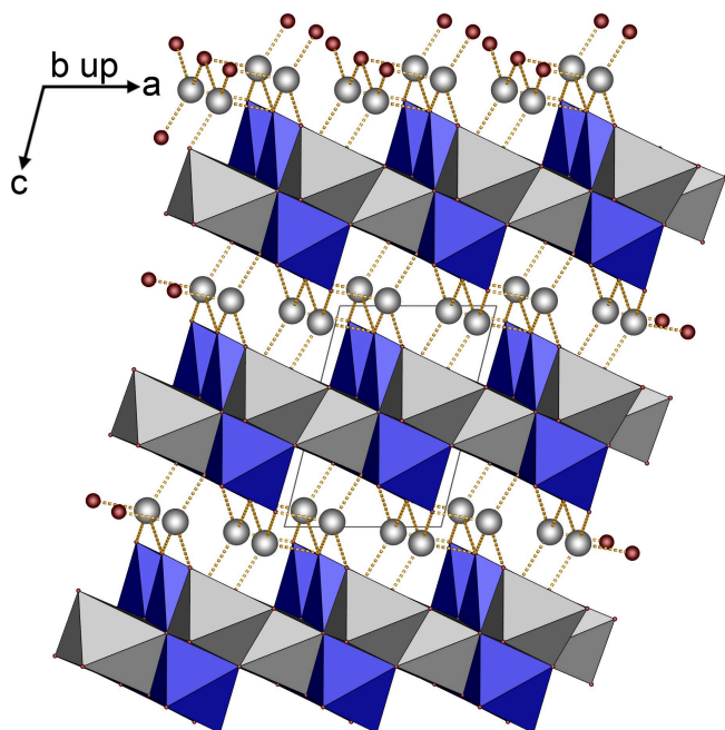
Figure 4. Layered structure of \text{Li}_2\text{WO}_4\text{-V} : Layers formed by edge sharing \text{LiO}_6 (grey) and \text{WO}_6 (blue) octahedra in the ab plane are connected via \text{Li}_4\text{O}_{10} building units along [001] ; oxygen atoms red, lithium atoms grey.
