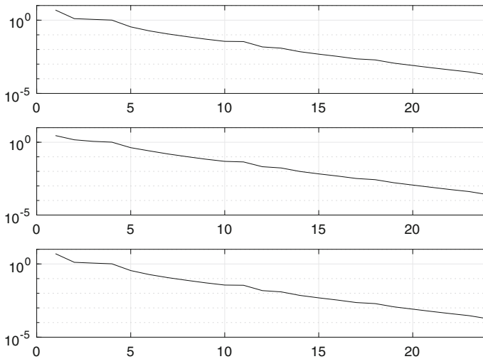
Fig. 7 Plots of \mu_{\hat{\Gamma}_N}/b_N (top), \sigma_{\hat{\Gamma}_N}/b_N (middle) and \hat{u}_{N,M}/b_N (bottom) (in \log_{10} -scale) for different sample sizes N (in \log_2 -scale), obtained by averaging over M batches. Note that all upscaled sequences converge to zero in our specific example, as expected
