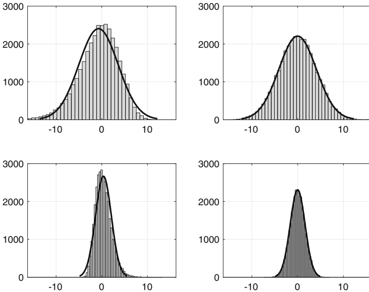
Fig. 1 Distribution of \sqrt{N}(\hat{f}_N^* - f^*) (upper half) and of \sqrt{N}(\hat{x}_N^* - x^*) (lower half) for N = 32 (left) and N = N^{\max} (right). Note that in the considered example approximate normality can already be obtained for small N
