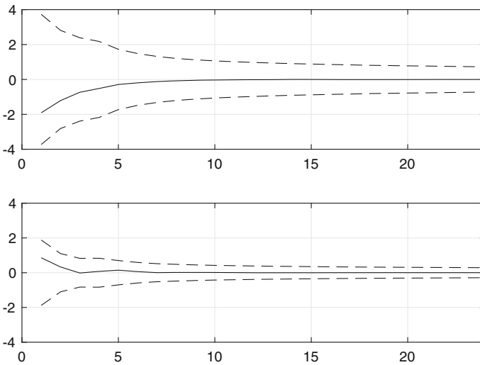
Fig. 5 Plots of the averages of \hat{f}_N^* (top) and \hat{x}_N^* (bottom) over M batches, centred at f^* and x^* , respectively, and upscaled by 1/b_N , for the different sample sizes N (in \log_2 -scale). The dashed lines represent the corresponding sample standard deviations, again upscaled by 1/b_N . Note that the negative bias of \hat{f}_N^* is clearly visible but vanishes asymptotically, as suggested by its order \mathfrak{o}(b_N)
