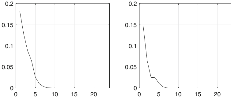
Fig. 4 Plots of \mathbb{P}((\hat{f}_N^* - f^*)/b_N \notin C^f) (left) and \mathbb{P}((\hat{x}_N^* - x^*)/b_N \notin C^x) (right) for the different sample sizes N (in \log_2 -scale), where the fixed confidence bands C^f and C^x are constructed according to Fig. 3. Note that these probabilities converge to zero as N \rightarrow \infty , as expected
