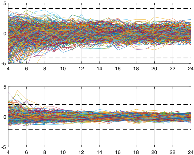
Fig. 3 Plots of the first 500 sample paths of (\hat{f}_N^* - f^*)/b_N (top) and (\hat{x}_N^* - x^*)/b_N (bottom) for the different sample sizes N (in \log_2 -scale). Note that for f^* the standard deviation of h(x^*, \xi) may be used as a good upper bound, while no such estimate is readily available for x^* , due to the unknown \alpha in the second-order growth condition (B2'). Therefore, a conservative estimate of \alpha = 2 has been used
