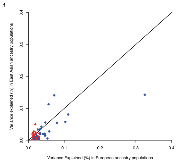
(y axes). c, d , Allele frequencies between ancestry groups, as in a and b . e, f , Comparison of the estimates of explained variance. In all plots, novel loci are in red and previously identified loci are in blue.
