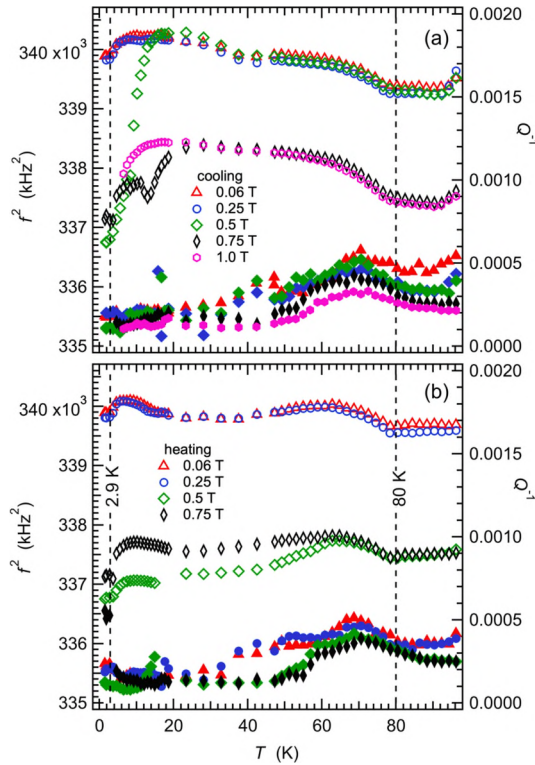
Fig. 7. f^2 and Q^{-1} variations for a resonance peak with frequency near 580 kHz in the same spectra as used to extract results for the 1170 kHz peak in Fig. 6a-e. The vertical broken line at 80 K marks the expected Néel temperature. An irreversible reduction in f^2 values occurred below \sim 15 K during cooling in a field of 0.5 T and the crystal became displaced from the sample holder below 6 K during cooling in a field of 1 T.
