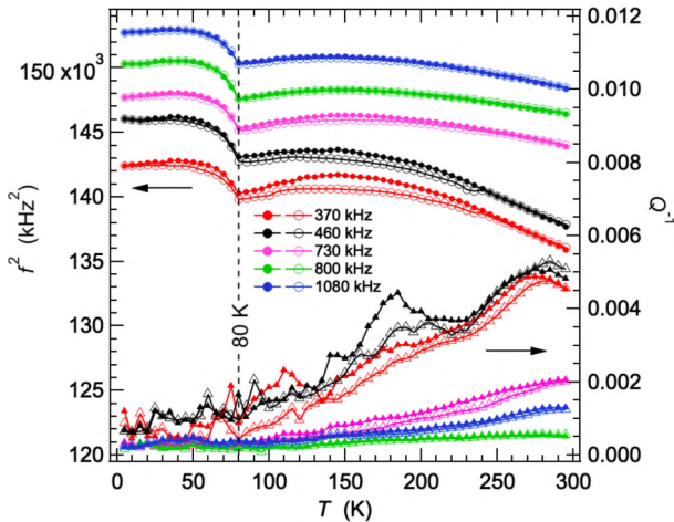
Fig. 12. f^2 and Q^{-1} variations as a function of temperature collected during cooling (filled symbols) and heating (open symbols) for several resonance peaks in spectra from a single crystal of Er 0.99 Zr 0.01 MnO 3 in the temperature interval 5–295 K. f^2 values for each resonance peak have been scaled arbitrarily along the y-axis in order to allow easy comparison of how they evolve.
