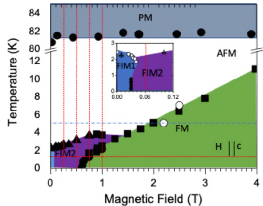
Fig. 1. Magnetic phase diagram of hexagonal \text{ErMnO}_3 for fields applied parallel to the crystallographic c -axis ( H//c ), adapted from [21]. PM = paramagnetic), FM = ferromagnetic (field aligned), \text{FIM}_1 = ferrimagnetic (multidomain), \text{FIM}_2 = ferrimagnetic (single domain state). Crystal 1 of the present study was the same crystal as used by Meier et al. [21] to determine boundaries between the stability fields of the magnetic structures. Discontinuous red lines mark the loci of temperature sweeps at constant magnetic field strength and magnetic field sweeps at constant temperature applied in RUS experiments described below. The blue dot-dash line marks the temperature/field trajectory applied to Crystal 2, though the field was not applied parallel to [001] in this case. (For interpretation of the references to colour in this figure legend, the reader is referred to the web version of this article.)
