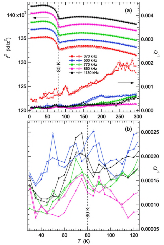
Fig. 10. Crystal 2. (a) f^2 (circles) and Q^{-1} (triangles) variations as a function of temperature for several resonance peaks in spectra collected in 5 K steps through the temperature interval 5–295 K. Open symbols = heating, filled symbols = cooling. f^2 values for each resonance peak have been scaled arbitrarily along the y-axis in order to allow easy comparison of how they each evolved. (b) Expansion of Q^{-1} data to show that there may still be a weak peak \sim 5 K below T_N .
