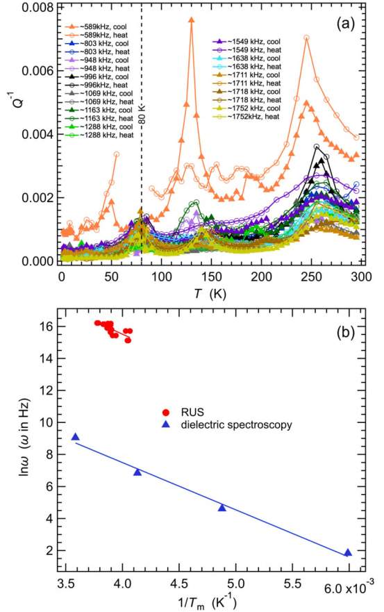
Fig. 5. (a) Q^{-1} variations from resonance peaks with the approximate frequencies listed in the captions, from spectra collected using the 12.4 mg piece of Crystal 1 with its long axis aligned parallel to the faces of the transducers. (b) Arrhenius plots of RUS data from fitting of the peaks near 250 K with Equation (1) and of dielectric spectroscopy data for the temperatures at which a peak in \tan\delta was observed by Ruff et al. [55].
