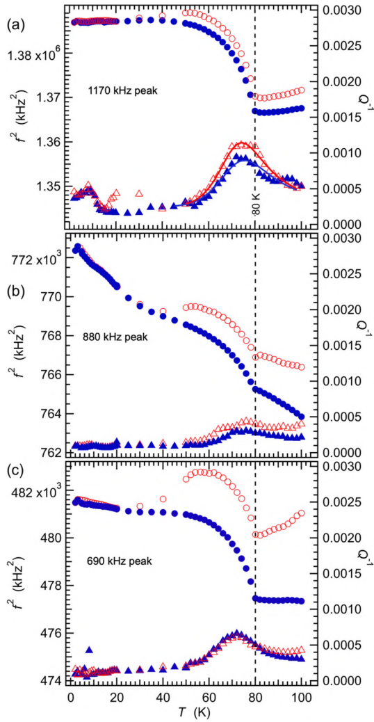
Fig. 4. Details of f^2 (open and filled circles) and Q^{-1} (open and filled triangles) variations for three representative resonance peaks in spectra collected during cooling (blue filled symbols), followed by heating (red open symbols), between 100 and 2 K from Crystal 1 (20 mg). The long axis was aligned perpendicular to the faces of the transducers. (a) The resonance near 1170 kHz shows the largest degree of stiffening ( \sim 1.5\% ) below T_N and the largest peak in Q^{-1} at \sim 75 K. An additional anomaly in Q^{-1} at \sim 9 K does not appear in data extracted from other resonance peaks and is considered to be an artefact. Solid curves are fits of Equation (1) to the data for Q^{-1} : E_a/Rr_2(\beta) = 595 \pm 13 K, T_m = 74.3 \pm 0.2 K, Q_m^{-1} = 0.00089 \pm 0.00001 (heating); E_a/Rr_2(\beta) = 550 \pm 33 K, T_m = 75.4 \pm 0.5 K, Q_m^{-1} = 0.00065 \pm 0.00003 (cooling). (b) Resonance with frequency near 860 kHz. This is representative of lower frequency resonances which showed the smallest change in trend of f^2 below \sim 80 K and the smallest peak Q^{-1} at \sim 75 K. (c) Resonance peak near 690 kHz. This displays most clearly the differences in f^2 values between cooling and heating at temperatures above \sim 30 K. (For interpretation of the references to colour in this figure legend, the reader is referred to the web version of this article.)
