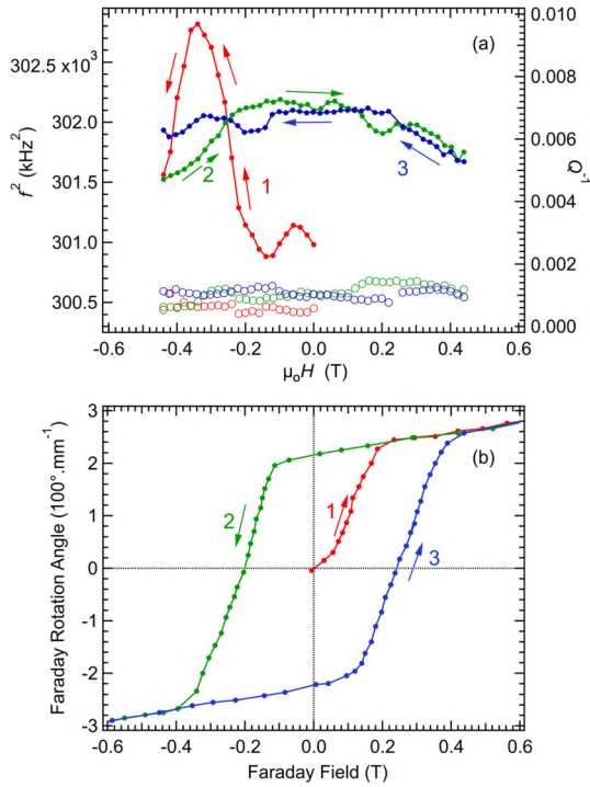
Fig. 9. (a) Hysteresis sequence at 2 K for f^2 (filled circles) and Q^{-1} (open circles) from a resonance peak with frequency near 550 kHz: 0 \rightarrow -0.44 T (first cycle), -0.44 T \rightarrow +0.44 T (second cycle), +0.44 \rightarrow -0.44 T (third cycle), in 0.02 T steps ( H/c ). (b) Magnetic hysteresis loop reproduced from Fiebig et al. [20] from a different crystal, also at 2 K and H/c . Faraday angle scales with magnetic moment. The full sequence was between +1.5 and -1.5 T, but only the segments between +0.6 and -0.6 T are shown.
