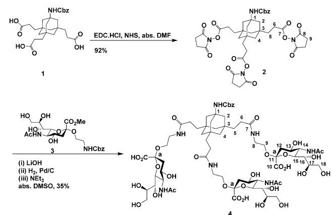
Scheme 1. Synthesis of adamantane core trivalent sialoside with an EG 1 spacer.
