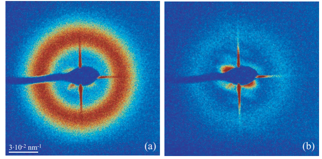
FIG. 9. Magnetic scattering data from the same sample in (a) unpumped and (b) pumped condition. The delay time between pump and probe laser was set to 1.2 ps and the pump fluence was 18 mJ/cm 2 . In both cases, three FEL shots were averaged at 1 Hz repetition rate to minimize the heating effect (Fig. 7). Speckles cannot be resolved due to the large illuminated area and the short sample-detector distance.
