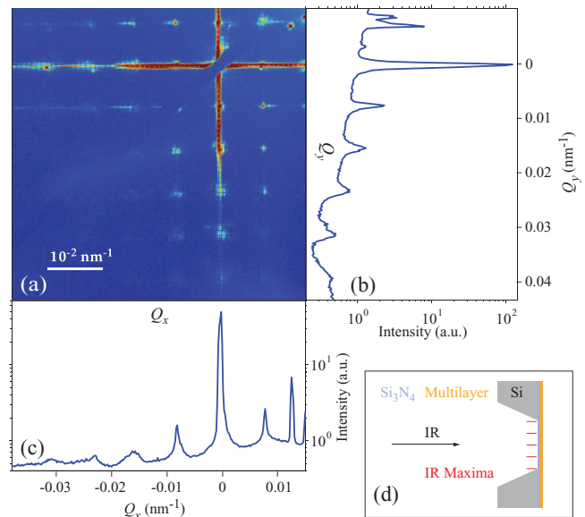
FIG. 11. CCD image (a) and line integration along the Q_x and Q_y directions (b) and (c) for a strongly pumped sample (120 mJ cm -2 not taking into account the lateral variation of the intensity). The structured pump laser has induced changes in the sample which are aligned in a grid. Therefore, the scattering also shows a grid-like structure and the periodicity yields the pump laser's wavelength. The high-intensity streaks intersecting at Q = 0 nm -1 are scattering from the membrane window. At higher magnification, fine dark lines become visible which are an artefact from the Ni mesh supporting the aluminum filter used in this experiment. See text for details. (d) The sample is irradiated from the groove side such that the pump-laser radiation is structured on the sample surface.
