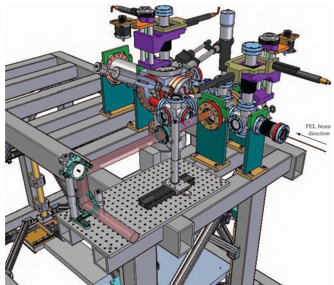
FIG. 4. Complete setup as used at BL3. Here, the chamber is shown mounted onto the base frame with all additional parts including the optical incoupling setup. See Figs. 2 and 3 to identify the various parts of the chamber.
