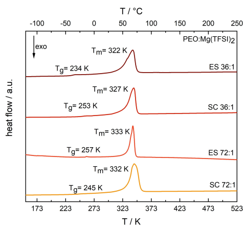
Figure 2. DSC curve of electrospun PEO:Mg(TFSI) 2 SPEs at different molar compositions and their fitted melting points T_m and glass transition temperatures T_g .
