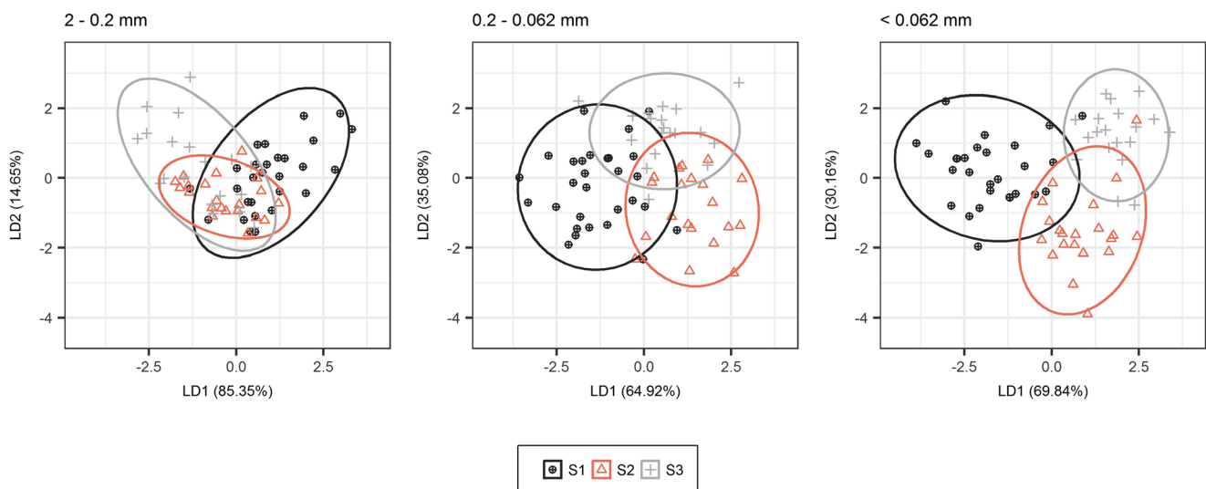
Fig. 3 LDA bi-plots of source reclassification using the selected elements from the statistical approach. Ellipses represent 90% confidence intervals
