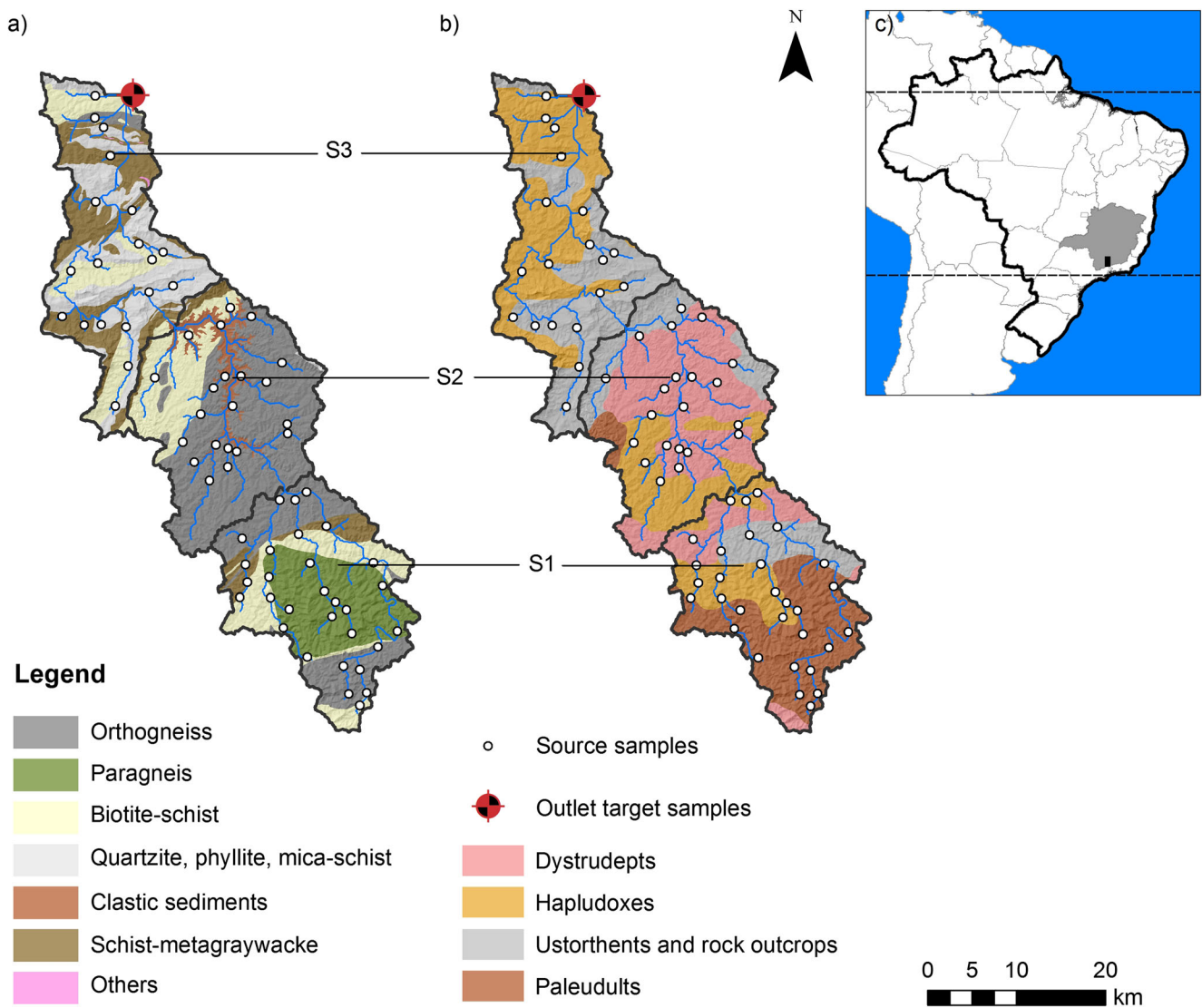
Fig. 1 Geological (a) and pedological (b) map of the Ingaí River basin, Brazil (c). S1: upper catchment; S2: mid catchment; S3: lower catchment. Adapted from CODEMIG–CPRM (2014) and FEAM (2010)
