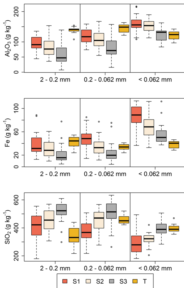
Fig. 7 Al 2 O 3 , Fe, and SiO 2 contents on source (S1: upper catchment; S2: mid catchment; S3: lower catchment) and target (T) sediments
