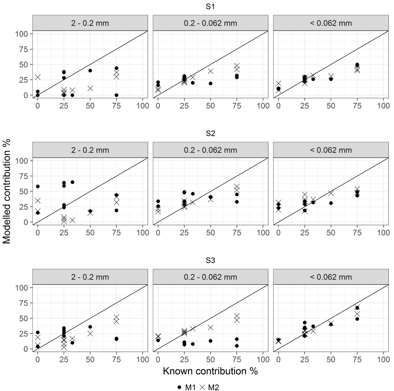
Fig. 5 Scatter plots of known and modeled source contributions of the artificial mixtures for each sediment size fraction. S1: upper catchment; S2: mid catchment; S3: lower catchment; M1: statistical element selection model; M2: knowledge-based element selection model
