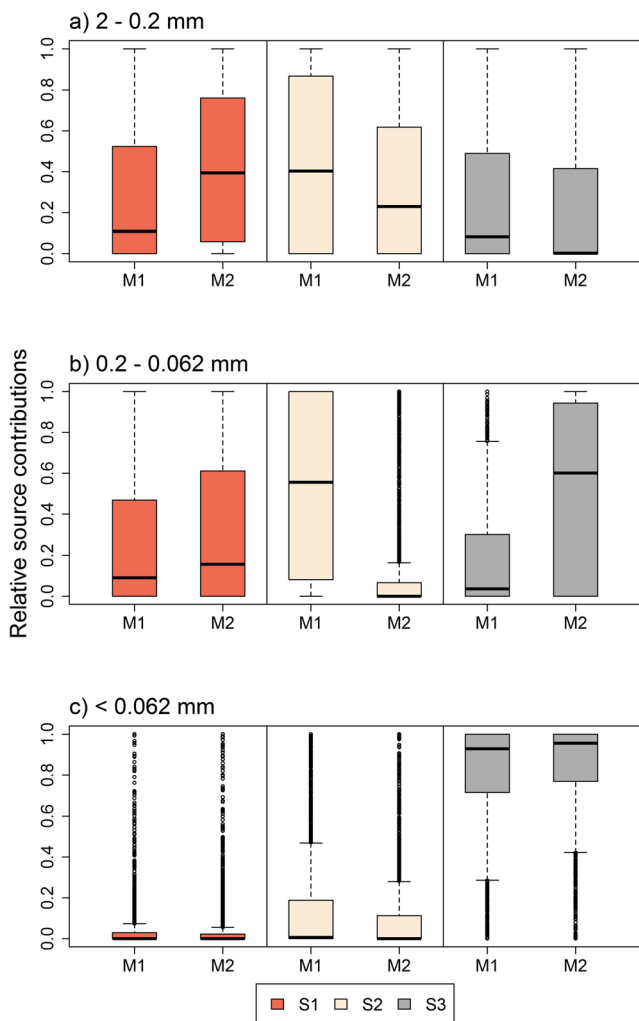
Fig. 6 Box plots of estimated source contributions based on the 2500 iterations of the Monte Carlo simulations. (a) Coarse fraction (2–0.2 mm). (b) Intermediate fraction (0.2–0.062 mm). (c) Fine fraction (<0.062 mm). S1: upper catchment; S2: mid catchment; S3: lower catchment; M1: statistical element selection model; M2: knowledge-based element selection model
