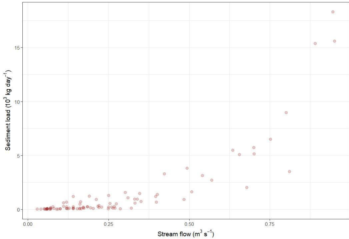
Fig. 2 Sediment load for streamflow less than 1 m³ s⁻¹.
