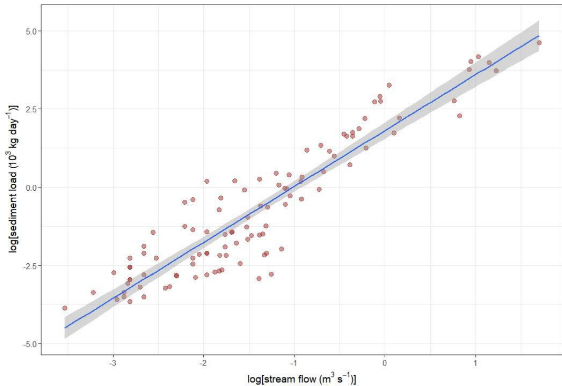
Fig. 5 Linear regression for log transformed streamflow and sediment load data. The grey area represents the confidence interval with 95% around the regression line.
