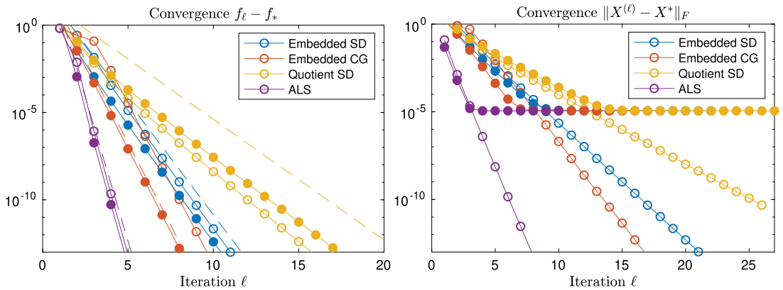
FIG. 1. Deterministic A with n = 50 , k = 5 and \delta = 0.95 \cdot \delta_{3k}^{\text{crit}} . Both panels show in open circles for zero noise ( \varepsilon = 0 ), and in closed circles for \varepsilon = 10^{-5} . Left panel shows in line the asymptotic convergence rate based on spectrum of Hessian.
