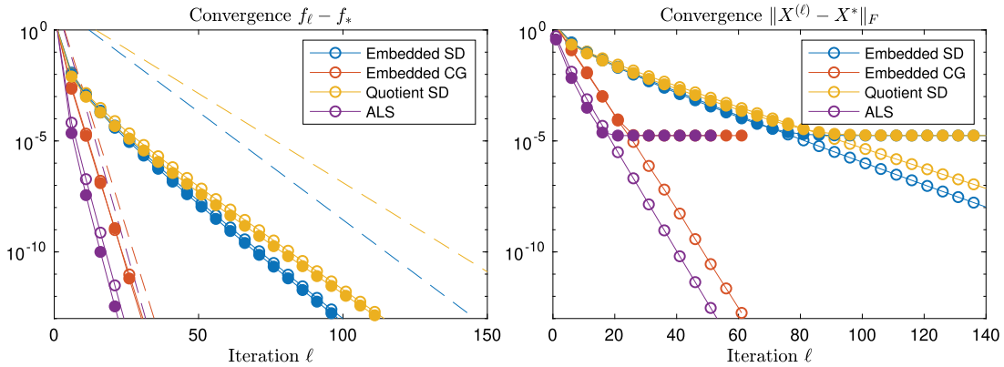
FIG. 2. Random Gaussian A with n = 50 , k = 5 , d = 5nk . Both panels show in open circles for zero noise ( \varepsilon = 0 ), and in closed circles for \varepsilon = 10^{-5} (every five iterations shown). Left panel shows in line the asymptotic convergence rate based on spectrum of the Hessian.
