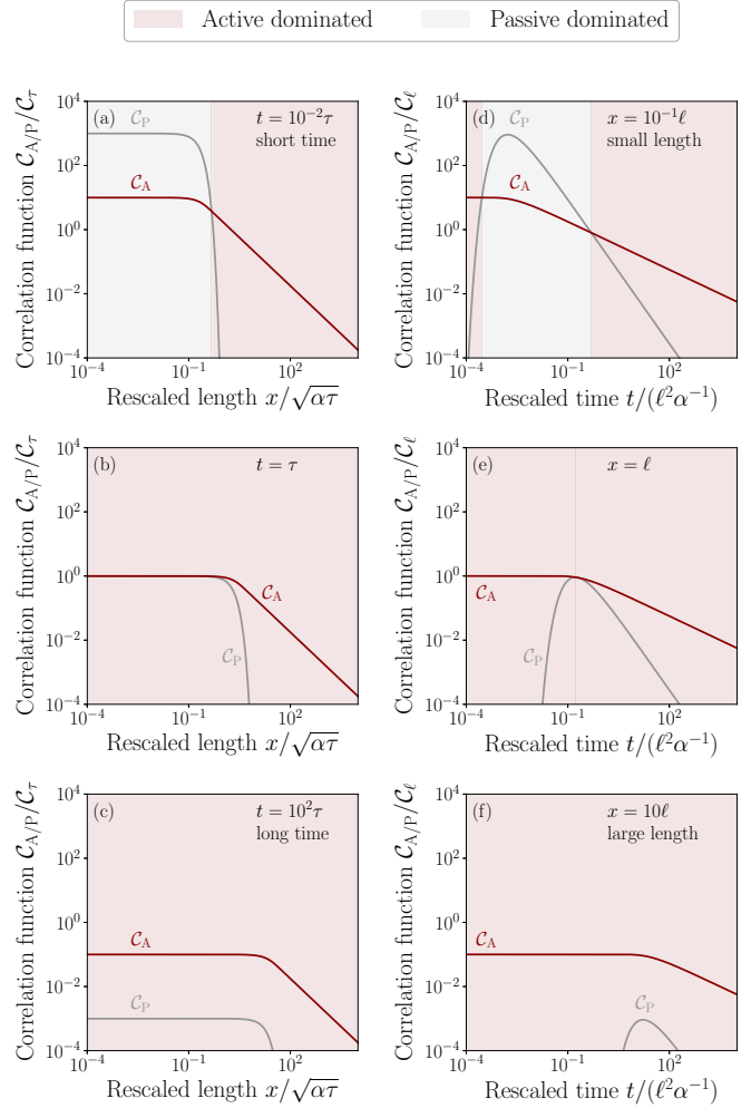
FIG. 2. Normalized two-point correlation functions C_P(x, t) (gray) and C_A(x, t) (red) for passive and active fluctuations. (a–c) Temperature correlations C_{A/P} normalized by C_\tau where C_\tau \equiv C_A(0, \tau) = C_P(0, \tau) with \tau given in Eq. (32), as function of normalized distance x/\sqrt{\alpha\tau} for t = 10^{-2}\tau (a), t = \tau (b) and t = 10^2\tau (c). (d–f) Temperature correlation C_{A/P} normalized by C_\ell where C_\ell \equiv C_A(\ell, \ell^2/6\alpha) = C_P(\ell, \ell^2/6\alpha) with \ell given in Eq. (34), as function of normalized time t/(\ell^2\alpha^{-1}) for x = 10^{-1}\ell (d), x = \ell (e), and x = 10\ell (f). The background shade indicates the dominant contribution to the correlation function: active (red), passive (gray). For the vertical line on panel (e), the contributions are equal.
