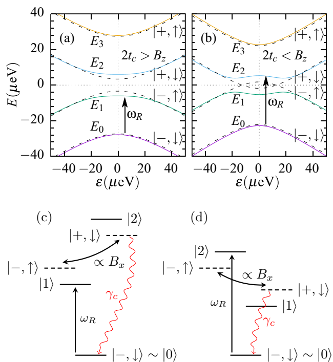
FIG. 2. (a),(b) Energy levels E_n ( n = 0, \dots, 3 ) as a function of the DQD detuning parameter \epsilon . The dashed lines are the energy levels without a magnetic field gradient ( B_x = 0 ). They correspond to the bonding (–) and antibonding (+) orbitals with spin \uparrow, \downarrow in the z direction, denoted by |\pm, \uparrow(\downarrow)\rangle . The arrow represents the transition driven by the probe field, at frequency \omega_R . Here, we choose the parameters B_z = 24 \mu\text{eV} and B_x = 10 \mu\text{eV} . For the tunnel coupling: (a) t_c = 15.4 \mu\text{eV} > B_z/2 and (b) t_c = 10.2 \mu\text{eV} < B_z/2 . (c),(d) Schematic representation of the \Lambda system that captures the essential dynamics in (a) and (b), respectively (near \epsilon = 0 ). If the orbital energy, \Omega = \sqrt{\epsilon^2 + 4t_c^2} , is near B_z , the levels |\pm, \uparrow\rangle and |\pm, \downarrow\rangle hybridize into the states |1\rangle and |2\rangle due to the magnetic field gradient, while the ground state is approximately unperturbed |0\rangle \sim |\pm, \downarrow\rangle . The wavy lines represent charge decoherence with rate \gamma_c .
