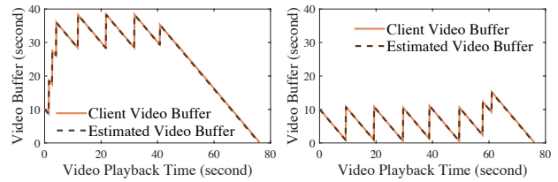
(a) Link capacity of 10 mbit/s (b) Link capacity of 512 kbit/s Fig. 4. Video Buffer over Playback Time in ES Scenario
