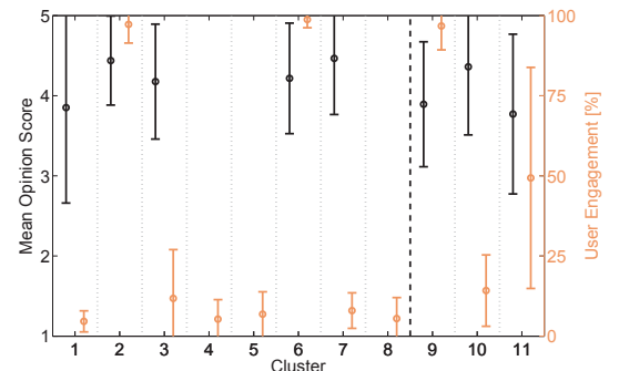
Fig. 4. MOS, mean user engagement, and their standard deviations of clusters.
