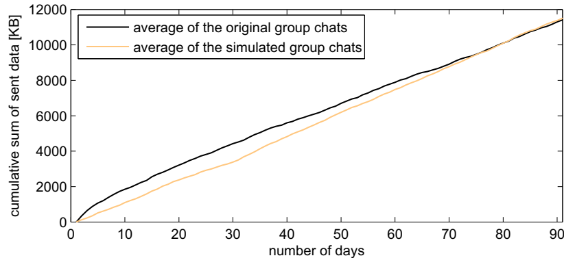
Fig. 8: Cumulative sum of sent KB per day of the original messaging histories and the simulation model
