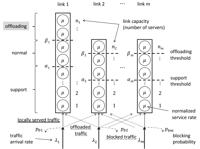
Figure 1: System model.
