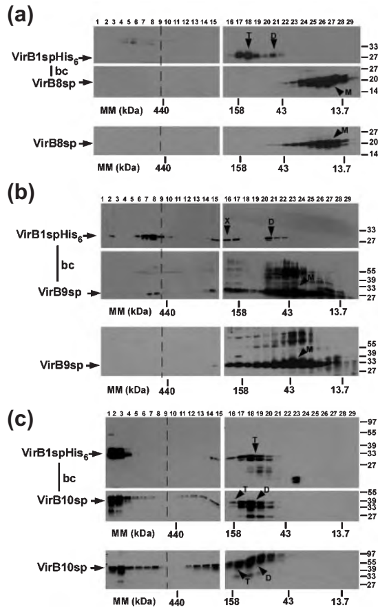
Fig. 2. Coelution of VirB1spHis 6 with other T4SS components: Superdex 200 gel filtration analysis of the molecular masses of VirB8sp (a), VirB9sp (b) and VirB10sp (c) expressed alone or from bicistronic vectors (bc) together with VirB1spHis 6 after overproduction and purification by affinity chromatography. After gel filtration, the proteins in the eluted 2 ml fractions were separated by SDS-PAGE followed by Western blotting and detection with specific antisera. Upper panels were probed with VirB1sp-specific antiserum, whereas lower panels were probed with antisera specific for VirB8sp (a), VirB9sp (b) and VirB10sp (c), respectively, as indicated by arrows. A dashed line marks the Superdex 200 void volume at >600 kDa. Arrowheads point to the expected size of monomeric (M), dimeric (D) and tetrameric (T) proteins. VirB1spHis 6 was detected in a complex of typical molecular mass (X), which was larger than the hexamer, exclusively after co-expression with VirB9sp. Molecular masses of SDS-PAGE marker proteins are given on the right in kDa; the elution of gel filtration reference proteins with their associated molecular masses (MM) from the Superdex 200 column is indicated below the chemoluminograms. All experiments were performed up to three times with similar results and the results of one set of representative experiments is shown.
