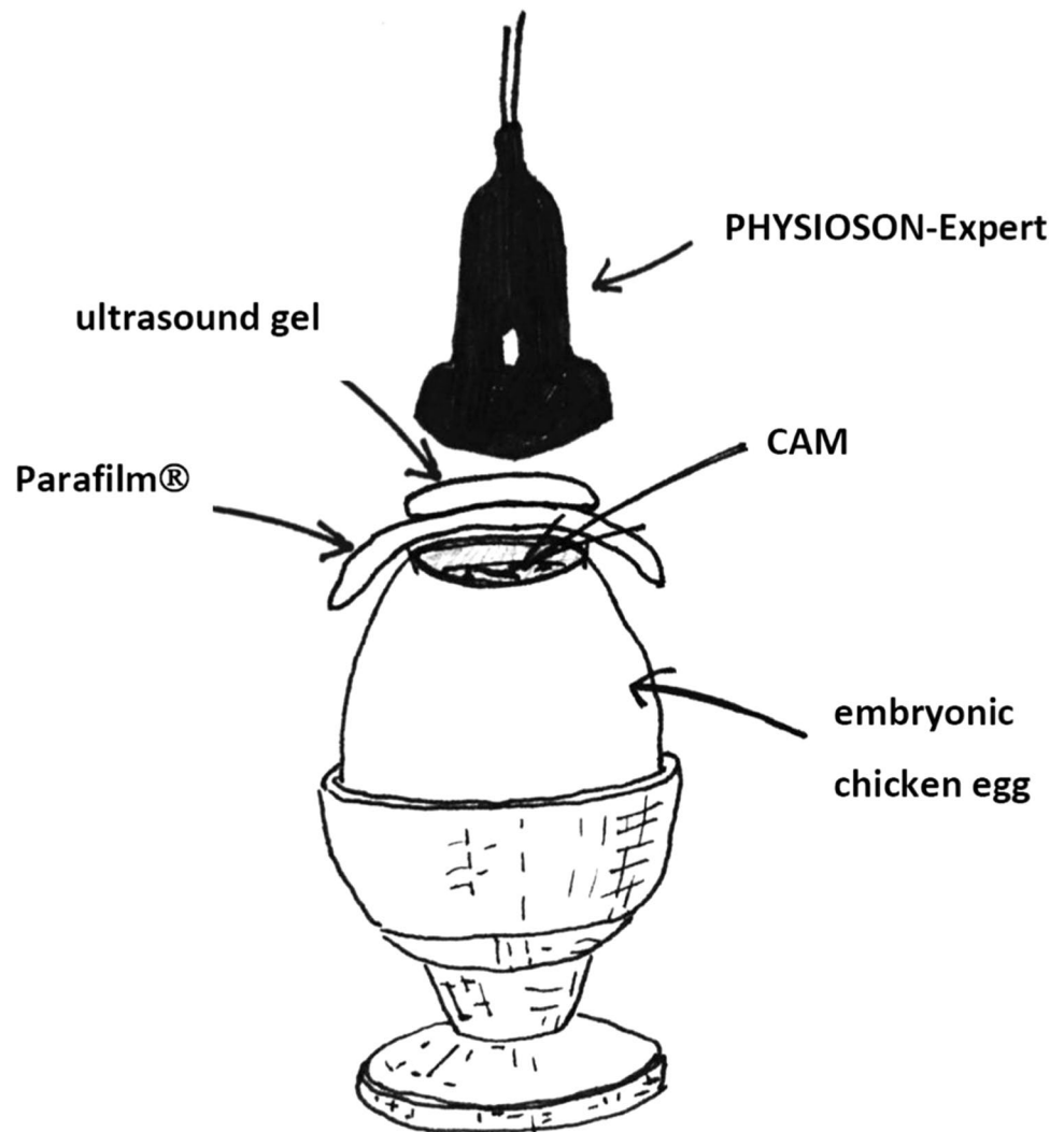
Fig. 1 Experimental setup during the ultrasound application to the CAM vessels with the exposed CAM through the egg-windowing covered with Parafilm® and ultrasound gel
