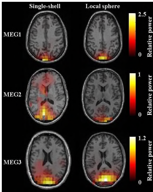
Fig. 3. Estimated sources of visually induced gamma-band activity on a single slice plot of a single-shell head model in the first column and local sphere in the second column for one of the representative subject. The first, second, and third row show sources as measured using MEG1, MEG2, and MEG3 sensor types respectively. The colorbars indicate the relative power change with respect to the baseline.
