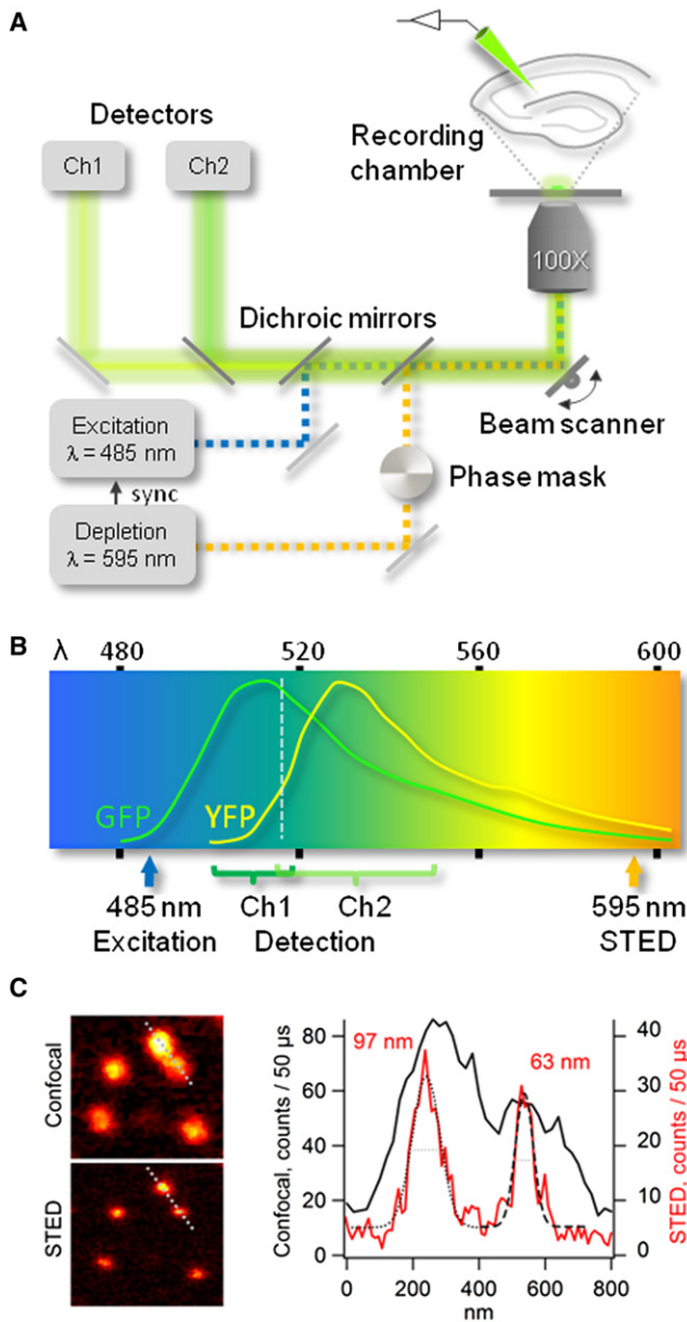
FIGURE 1 (A) Scheme of custom-built STED microscope. The lasers for excitation (485 nm) and depletion (595 nm) are synchronized ( small arrow ) and their beams are brought into coincidence and scanned across the brain-slice cultures in the recording chamber. A vortex phase plate imposes the doughnut shape on the depletion beam. Emitted fluorescence from the sample is descanned and split into the two detection channels on either side of the 514-nm long-pass dichroic mirror placed in front of channel 2. Removing this long-pass filter reverts the STED setup to single-channel detection. (B) Excitation and excited-state depletion is separated spectrally by >100 nm, leaving open a wide spectral range for fluorescence detection. The emission spectra for GFP and YFP are shown, illustrating their differing relative distribution on either side of the 514-nm long-pass filter ( dotted line ) that allows linear spectral unmixing of the two detection channels. The emission spectra for Alexa Fluor 488 and Calcein green are very similar to that of GFP (not shown). (C) Imaging the same frame of fluorescent beads by confocal and STED microscopy reveals the gain in spatial resolution by STED. Plots of the bead intensity profiles corresponding to the dotted lines in the images at left are depicted in the graph at right. The gain in resolution achieved by STED ( red line ,
