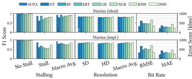
Fig. 9. F1 scores for stalling/resolution classification, error scores (RMSE and MAE) for bit rate inference.
