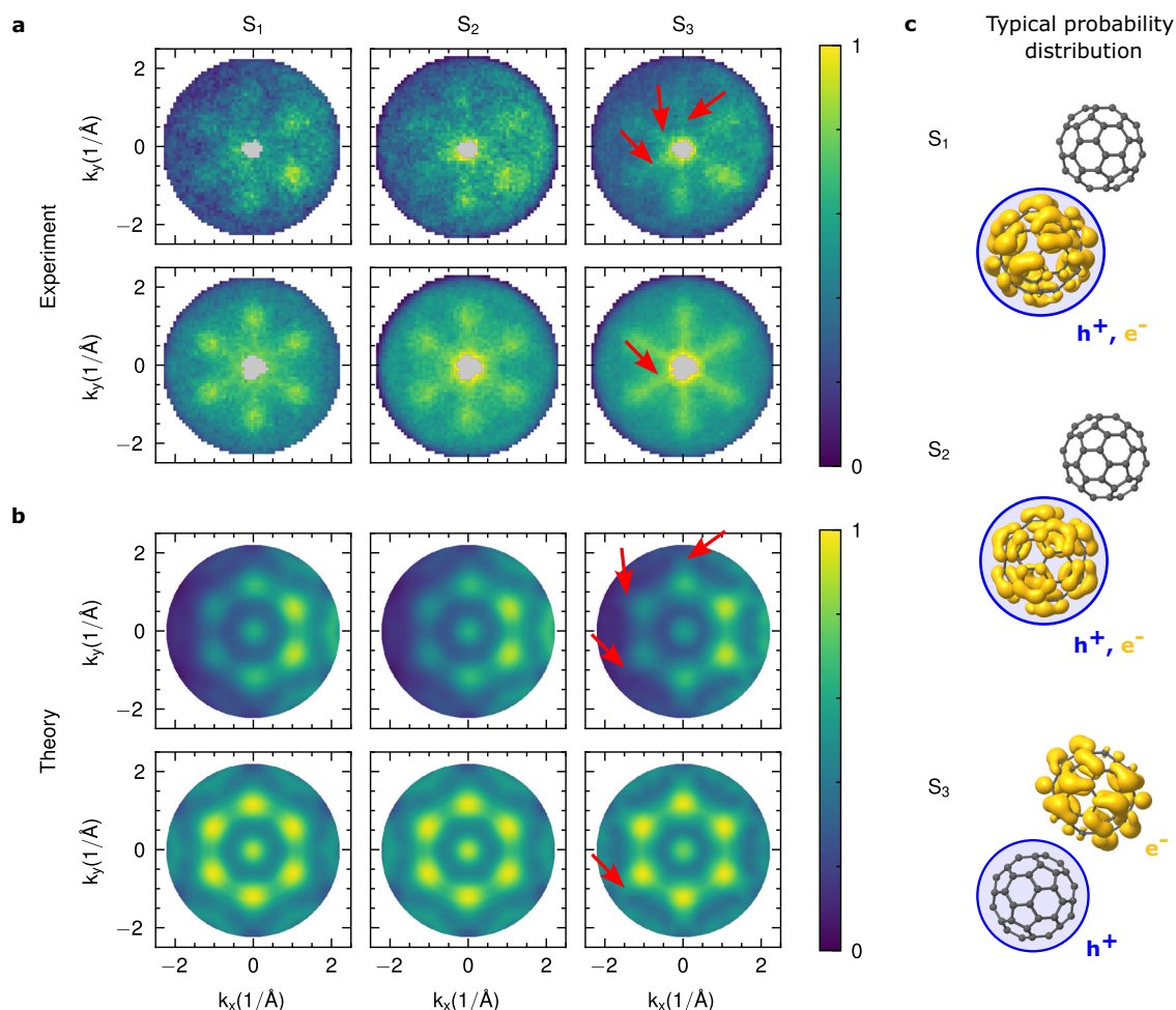
Fig. 4 | Photoelectron momentum distribution and exciton real space probability distribution of the three exciton bands observed in C 60 . a Comparison of the experimental momentum maps acquired for the S 1 , S 2 and S 3 , with the b predicted momentum maps retrieved from GW +BSE. The top rows show the raw data and the bottom rows 6-fold symmetrized data, respectively. Note that the
