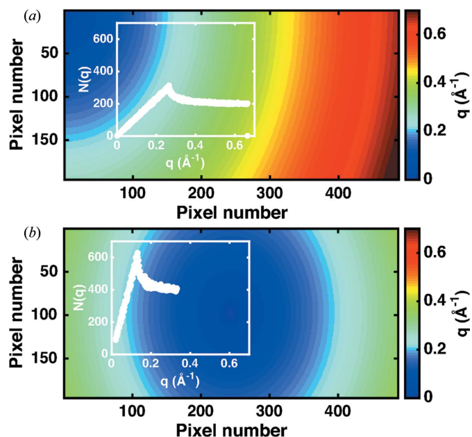
Figure 3 Measurement geometry and the number of pixels per q bin. Assignment of the pixels in two dimensions to q bins for different positions of the beam centre on a PILATUS 100K detector, with an X-ray energy of 17.4 keV and a sample–detector distance of 1.11 m. (a) Configuration with the beam centre aligned on the top left corner of the detector. (b) Setup with the beam centred on the detector. The insets show the resulting pixels per q bin N(q) . Further beam centre positions are depicted in Fig. S4.
