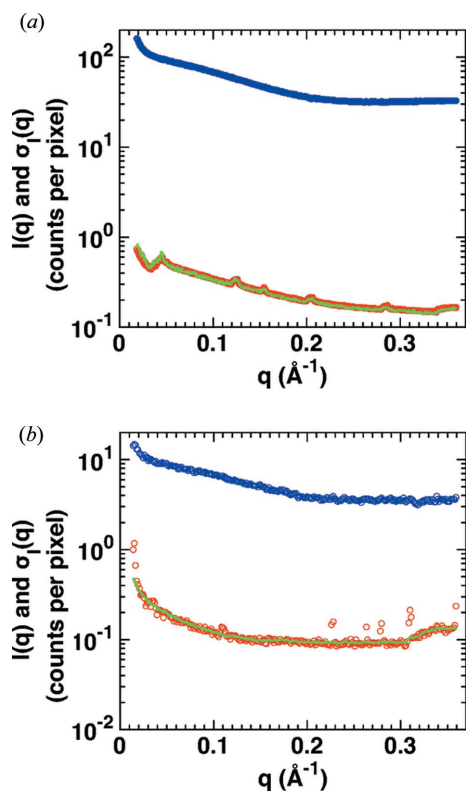
Figure 2 Counting statistics of SAXS profiles before buffer subtraction. SAXS measurements of cytochrome c (at 8 \text{ mg ml}^{-1} ) at (a) a synchrotron source (exposure time 1 s; BM29, ESRF, Grenoble) and (b) an in-house source (Bruetzel et al. , 2016) (exposure time 2 h; Department of Physics, LMU Munich). Scattering profiles of the protein samples after circular averaging are shown as blue circles; the corresponding standard errors of the mean \sigma_s computed from the counts in the individual pixels [equation (2)] are shown as red circles. The green line is the square root of the intensity divided by the number of pixels per q bin \{\sigma_s(q) = [I_s(q)/N(q)]^{1/2}\} .
