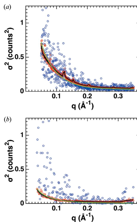
Figure 4 SAXS measurement errors after buffer subtraction. SAXS measurement of cytochrome c (24 mg ml -1 ) obtained (a) at a synchrotron source (BM29, ESRF, Grenoble) and (b) from our in-house source (Department of Physics, LMU Munich). The propagated standard errors for the buffer-subtracted measurement from single exposures of sample and buffer are shown as red symbols. The black lines are co-plots of equation (8) with the red data, using the exact number of pixels per q bin for the respective setups and determining the contrast factor c by dividing the buffer by the sample intensity at q_{\text{arb}} = 0.2 \text{ \AA}^{-1} [synchrotron: c = 0.69 , I(q_{\text{arb}}) = 14.20 ; in-house setup: c = 0.68 , I(q_{\text{arb}}) = 2.30 ]. The green lines show fits of equation (10) to the data, with k as a free fitting parameter (synchrotron: k = 6104 ; in-house setup: k = 4298 ). The blue data points show the variance in the intensity determined from repeat exposures (synchrotron: ten exposures of 4 s each; in-house setup: three exposures of 3 h each) for comparison.
