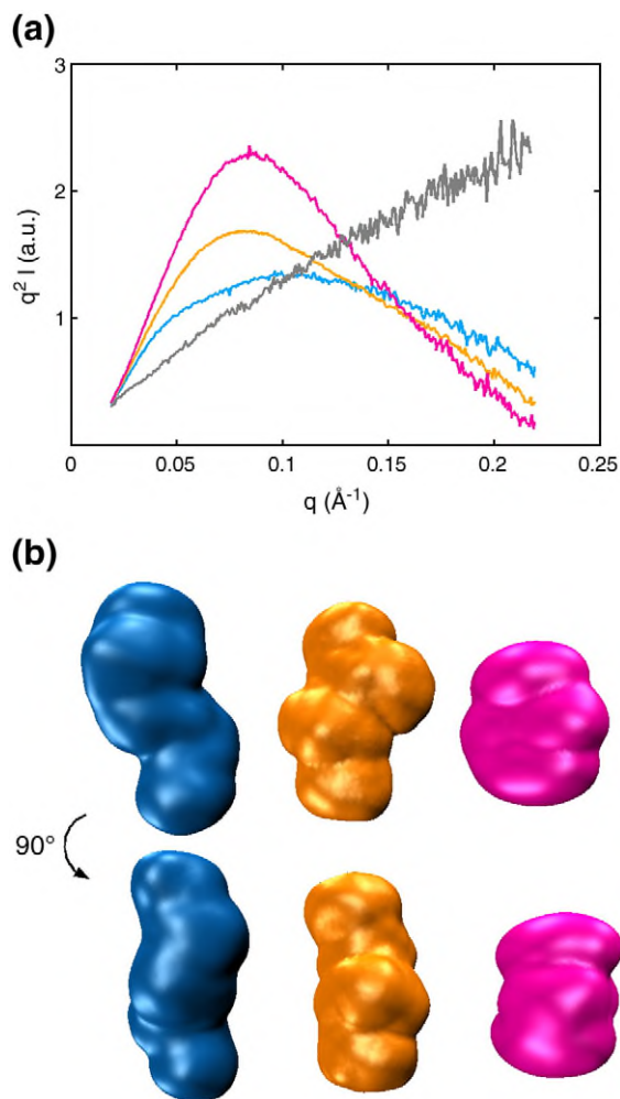
Fig. 2. SAXS data for the structure of the TPP riboswitch aptamer in the absence of \text{Mg}^{2+} and TPP (blue), defined as the ‘unfolded’ state; in 10 mM \text{Mg}^{2+} but no TPP (orange), defined as the ‘intermediate’ state; and in 10 mM \text{Mg}^{2+} and 10 mM TPP (pink), defined as the ‘folded’ state. Data are also shown for the denatured riboswitch in 7 M urea (gray). (a) SAXS profiles in Kratky representation [ q^2 I(q) versus q for the full-scattering profile] under different solution conditions. (b) Low-resolution bead models for the TPP riboswitch in its unfolded, intermediate, and folded states, obtained from the SAXS profiles in (a). See Materials and Methods for details on structure reconstruction.
