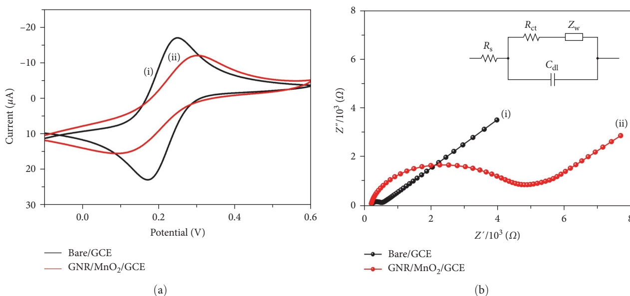
FIGURE 4: Electrochemical analysis of (a) CV and (b) EIS spectra of (i) bare GCE and (ii) GNR/MnO 2 /GCE in 0.1 M KCl with 2 mM (Fe(CN) 6 ) 3- at scan rate of 50 mV s -1 . Inset: Randles' equivalent circuit.
