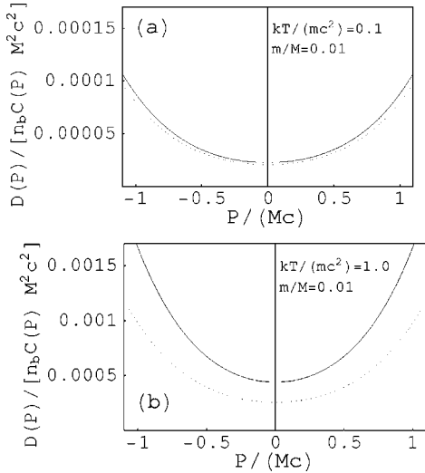
FIG. 4. Relativistic diffusion coefficients D(P) calculated numerically for different heat bath distributions f_b^l(p) for (a) weakly and (b) strongly relativistic heat. The solid lines refer to a standard Jüttner distribution with \eta=0 , and the dotted lines to \eta=1 in Eq. (17b).
