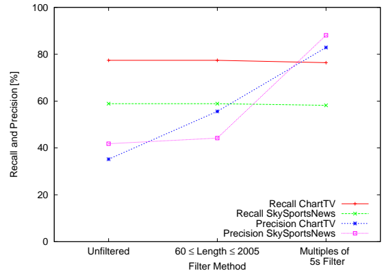
Figure 4: Content related filter methods.
