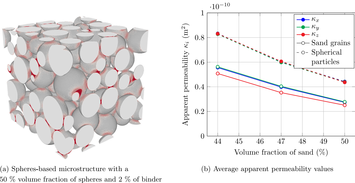
Fig. 14. Permeability computations on sand-based and spheres-based microstructures.
