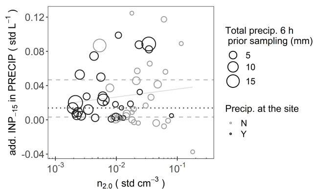
Figure 4. Difference between [\text{INP}_{15}] in precipitating (PRECIP) air masses and the function fitted to the non-precipitating (NON-PRECIP) air masses (additional [\text{INP}_{15}] in PRECIP) versus [n_{2,0}] . The median difference is 0.014 \text{ std L}^{-1} (black dotted line), and the lower and upper quartiles are 0.003 and 0.047 \text{ std L}^{-1} , respectively (grey dashed lines). The linear fit (grey solid line) is weakly positive but not significant (Pearson correlation test, R = 0.0027 , and p = 0.98 ). The circle area is proportional to the amount of precipitation along the last 6 h of the trajectory prior to sampling. Black circles are for samples precipitating at Weissfluhjoch.
