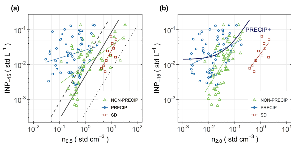
Figure 3. Cumulative concentrations of ice-nucleating particles active at -15^\circ\text{C} [ \text{INP}_{-15} ] (a) versus [ n_{0.5} ] and (b) versus [ n_{2.0} ] for PRECIP (blue circles), NON-PRECIP (green triangles), and SD (red squares) air masses. Power functions (solid lines) for each type of air mass based on [ n_{0.5} ] and [ n_{2.0} ] are shown. An additional preliminary parameterisation for precipitating air masses based on [ n_{2.0} ] is shown (PRECIP+, thick dark blue line). It is the same as for non-precipitating air masses but with an added constant equivalent to 0.014 \text{ INPs L}^{-1} . The corresponding equations and R^2 values are shown in Table 1. The grey lines show the D15 parameterisation extrapolated to -15^\circ\text{C} and corrected for the difference between physical and aerodynamic diameters (see the “Material and method” section) with three different calibration factors (Eq. 1): \text{CF} = 3 (dashed), \text{CF} = 1 (continuous), and \text{CF} = 0.086 (dotted). The latter value was the best fit found by Schrod et al. (2017) for Saharan dust above Cyprus.
