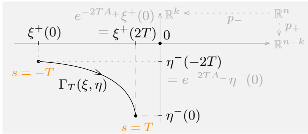
Fig. 3 Infinitesimal gluing isomorphism \Gamma_T \in \mathcal{L}(\mathbb{E}^+ \times \mathbb{E}^-, \mathbb{E}_T) ; cf. (3.29)
