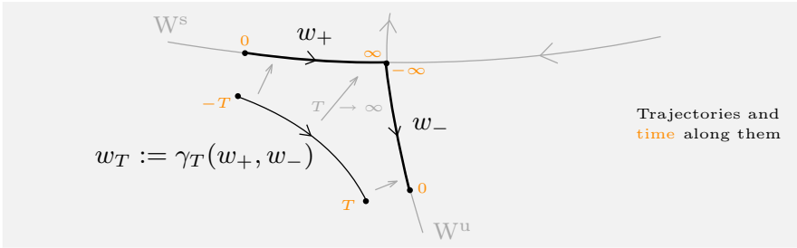
Fig. 1 Convergence of local gluing ev_T \circ \gamma_T(w_+, w_-) \xrightarrow{T \rightarrow \infty} ev(w_+, w_-)
