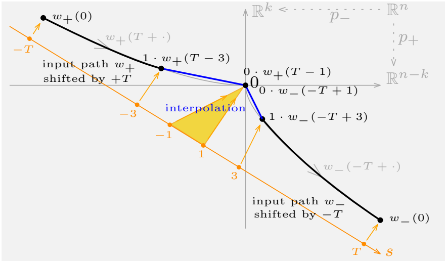
Fig. 2 Pre-glued path w_T(s) := \mathcal{P}_T(w_+, w_-)(s) for s \in [-T, T]
