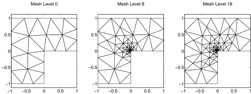
FIG. 5.1. Ex. 1: The initial mesh (left) and the meshes after 8 (middle) and 18 (right) adaptive refinement steps ( k = 4 and \Theta = 0.1 ).
