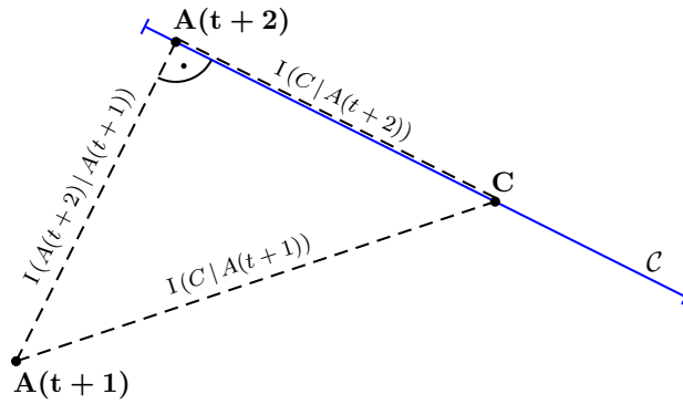
Figure 1: Geometric interpretation of the three-points property (Lemma 5.1) in the two-dimensional Euclidean space. The three-points property can be interpreted as the Pythagorean theorem with I-divergence as the squared Euclidean distance.
