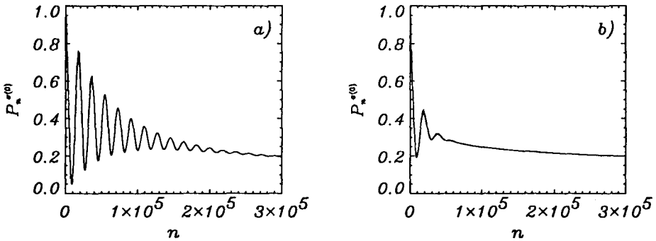
Fig. 7. Transient tunneling between limit cycles, in terms of the time evolution of P_n^{s(t)} over the first 3 \times 10^5 time steps, at parameter values as in Fig. 6, but with \gamma = 5 \times 10^{-6} , for initial states prepared as coherent states located at either one of the maxima of the stationary Husimi distribution in the left well, i.e., at p = 0 and (a) x = -7.5 , (b) x = -4.2 .
