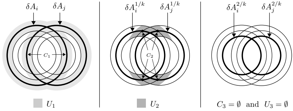
Figure 2.1: Saturation and missing product structures after smoothing
