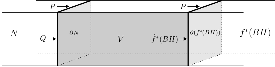
Figure 4.3: Boundary of the singular P -bordism W
