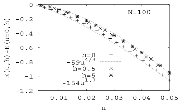
Fig. 2 Energy gain versus dimerization for \Delta = -1 and various impurity strengths.
