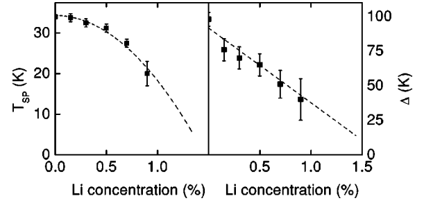
FIG. 4. Variation of the transition temperature T_{SP} and energy gap \Delta(0) with lithium concentration. The dashed line in the left graph represents a fit according to T_{SP}(x)\propto a-bx^2 ; the dashed line in the right graph is a guide to the eye.
