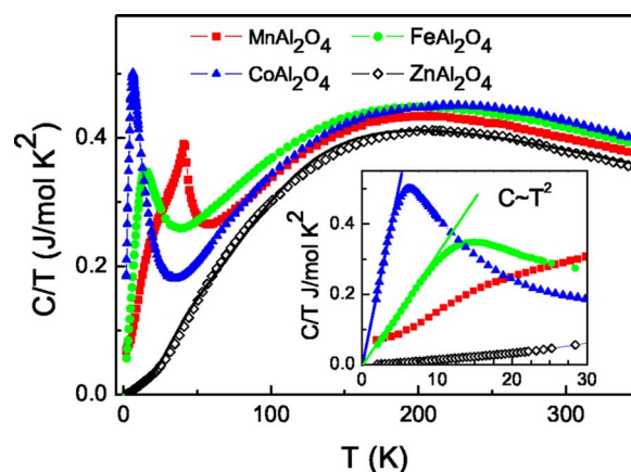
FIG. 7. (Color online) Heat capacities of M\text{Al}_2\text{O}_4 , M=\text{Mn} (■), \text{Fe} (●), \text{Co} (▲), and \text{Zn} (◇) plotted as C/T vs T . The inset shows the low-temperature values on an enlarged scale, where the quadratic regime C \sim T^2 is indicated by straight lines.
