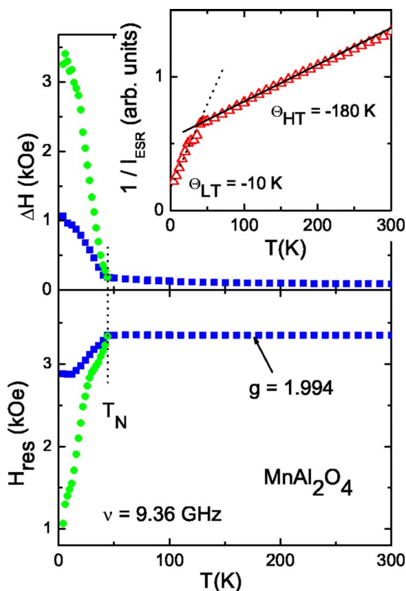
FIG. 6. (Color online) Resonance field H_{\text{res}} (lower frame) and linewidth \Delta H at resonance absorption (upper frame) as determined in \text{MnAl}_2\text{O}_4 by ESR measurements at X -band frequency. The inset in the upper frame shows the inverse ESR intensity 1/I_{\text{ESR}} vs temperature. The solid and dotted lines indicate high-temperature and low-temperature CW laws with the corresponding CW temperatures \Theta_{\text{HT}} and \Theta_{\text{LT}} .
