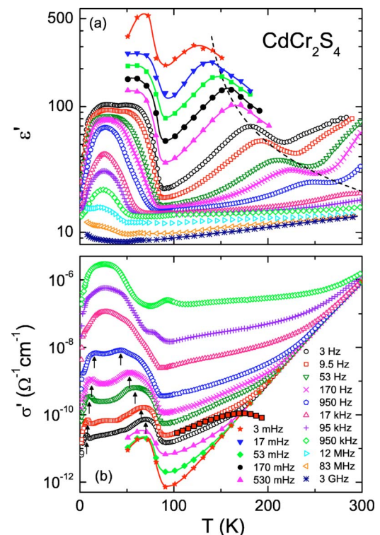
FIG. 1. (Color online) Temperature dependence of \epsilon' (a) and \sigma' (b) of CdCr 2 S 4 for various frequencies [in (b) not all frequencies are shown]. The solid lines are drawn to guide the eyes. The dashed line in (a) indicates the static dielectric susceptibility following a Curie-Weiss like law with a characteristic temperature of 130 K. The closed squares in (b) show \sigma'(\nu) at 9.5 Hz after subtraction of the dc conductivity. The arrows in (b) indicate the relaxation peaks below T_c .
