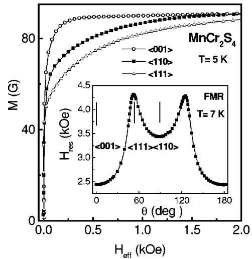
FIG. 4. Magnetization versus internal magnetic field H_{\text{eff}} = H - NM (here N is the demagnetizing coefficient, determined from the M(T) curves in low fields close to T_C ) for different crystallographic directions in a \text{MnCr}_2\text{S}_4 single crystal (sample 16-13) at 5 K. Inset: Angular dependence of the ferromagnetic resonance field for a disklike single-crystalline \text{MnCr}_2\text{S}_4 sample (16-13d3) within the (110) plane at 7 K. Solid lines are guides to the eye.
