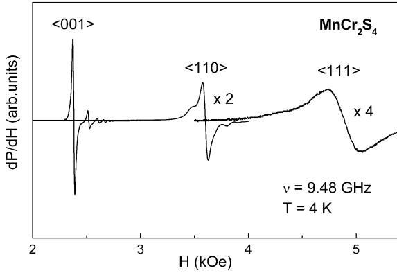
Fig. 1. ESR spectra for a \text{MnCr}_2\text{S}_4 single crystal (disk I) at 4 K for the magnetic field applied within the (110) plane along the three principal cubic axes.
