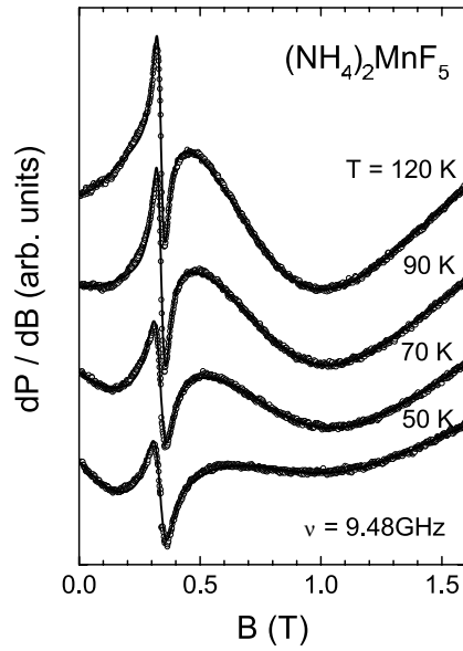
Figure 3. The temperature dependence of the ESR spectra of (\text{NH}_4)_2\text{MnF}_5 for measuring geometry B \parallel \vec{a} and \vec{h} \parallel \vec{b} . At T = 120 K, the full curve corresponds to a fit of a narrow and a broad resonance according to equation (1). At lower temperatures a good fit to the data could only be achieved by assuming an additional splitting of the broad resonance into two Lorentzian lines.
