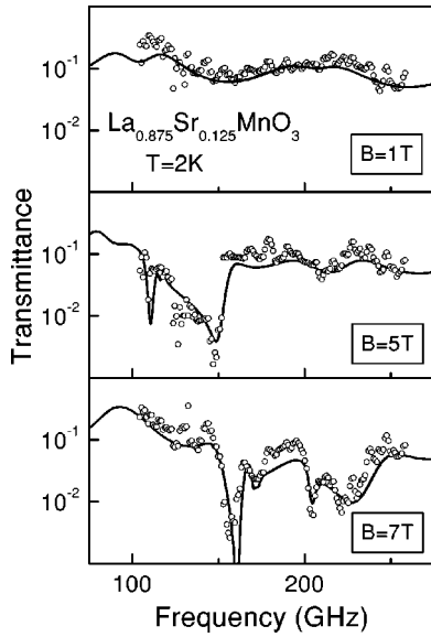
FIG. 5. Frequency-dependent transmittance of a 0.194-mm-thick \text{La}_{0.875}\text{Sr}_{0.125}\text{MnO}_3 single crystal in the Faraday geometry. Upper panel: B=1 T; the FMR mode is below the frequency range of the experiment. Middle ( B=5 T) and lower ( B=7 T) panels: the complicated character of the FMR spectra is due to interference effects and Faraday rotation. Symbols, experiment. The lines represent the calculated transmittance of the platelet-shaped sample assuming a parallel orientation of the polarizer and analyzer. The model parameters are the same for all curves: g=2 , M \approx 4 \mu_B/\text{Mg atom} , \epsilon^* = 56 + i5.7 , FMR linewidth \delta = 0.1 \text{ cm}^{-1} .
