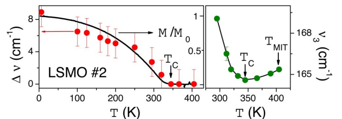
FIG. 5. Left panel: Splitting \Delta\nu = \nu_2 - \nu_1 between the eigenfrequencies of the two external modes at various temperatures (full circles). The solid line is the temperature dependent magnetization of LSMO No. 2. Right panel: Temperature dependence of the frequency of the new mode \nu_3 . At T_C the direction of the shift is reversed. Beyond T_{\text{MIT}} the phonon spectrum is invariant with respect to T .
