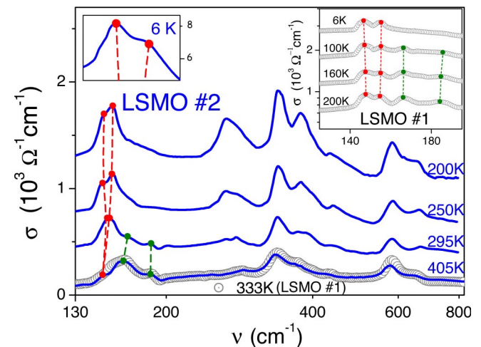
FIG. 3. Temperature-dependent optical conductivity ( \sigma ) spectra of LSMO No. 2 (solid lines), with a spectral resolution \sim 1 \text{ cm}^{-1} on a logarithmic frequency scale. We found similar spectra for LSMO No. 1 (open circles at 333 K and right inset), except for a reduction of the respective absolute values and a slightly reduced temperature scale for the evolution of the external modes. The vertical lines connect the maxima of the external modes. Left inset: At 6 K the splitting of the external modes is strongest.
