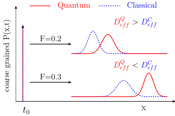
FIG. 5: The influence of the quantum corrections on the evolution of the coarse grained probability density function P(x,t) (see discussion in [22]) is illustrated for the same set of parameters as in Fig. 2 and for different forces F = 0.2 and 0.3 . Note that in the quantum case the velocity is always larger; therefore, the maximum of the density is located at a more distant position as compared to the classical case. The width of the density differs depending on the driving parameters and thereby reflects the effective diffusion strength.
