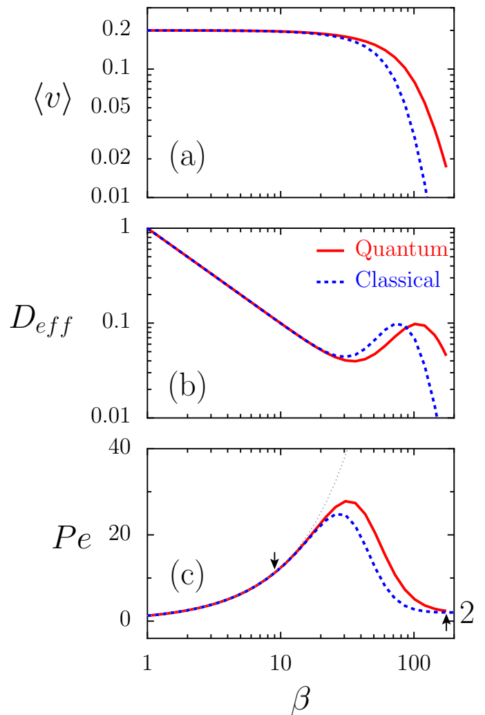
FIG. 3: Average velocity (a), effective diffusion (b) and Peclet number (c) versus the inverse temperature \beta . The chosen parameters are: bias F = 0.2 , potential parameters \varepsilon = 100 and \Delta = 10 . The two arrows in panel (c) mark the characteristic temperatures where the system starts to markedly deviate from the classical behavior (see text for details). The region of intermediate temperatures is located between the downward and upward pointing arrows. It bridges between the regions of freely sliding Brownian particle dynamics, characterized by the Peclet number Pe = FL\beta (see the thin, dotted line in (c)) and the Poisson like behavior with Pe = 2 . Within this region the Peclet number assumes its maximal value.
