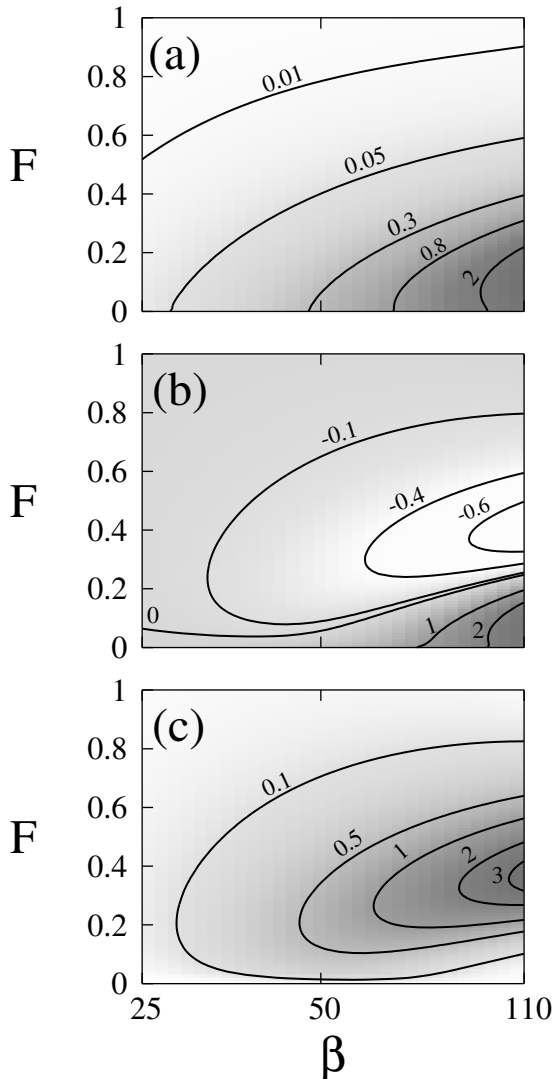
FIG. 4: The influence of quantum corrections are illustrated as a function of bias F vs. inverse temperature \beta by the relative difference between the quantum ( Q ) and the corresponding classical ( C ) values of the current ( \langle v \rangle^Q - \langle v \rangle^C )/ \langle v \rangle^C (a), the effective diffusion (D_{eff}^Q - D_{eff}^C)/D_{eff}^C (b) and the Peclet number (Pe^Q - Pe^C)/Pe^C (c), respectively. The positive values of the depicted quantities indicate the relevant role of quantum effects.
