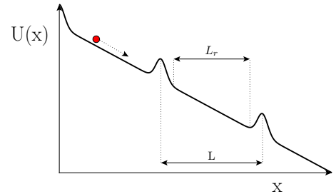
FIG. 1: Schematic picture of the Brownian particle in the tilted periodic potential U(x) = V(x) - Fx , defined in (1) and (17) below, plotted for the following set of parameters: \Delta = 10 , \varepsilon = 10 , F = 0.2 , L denotes the period the potential V(x) and L_r stands for the length of free slide between the barriers.
