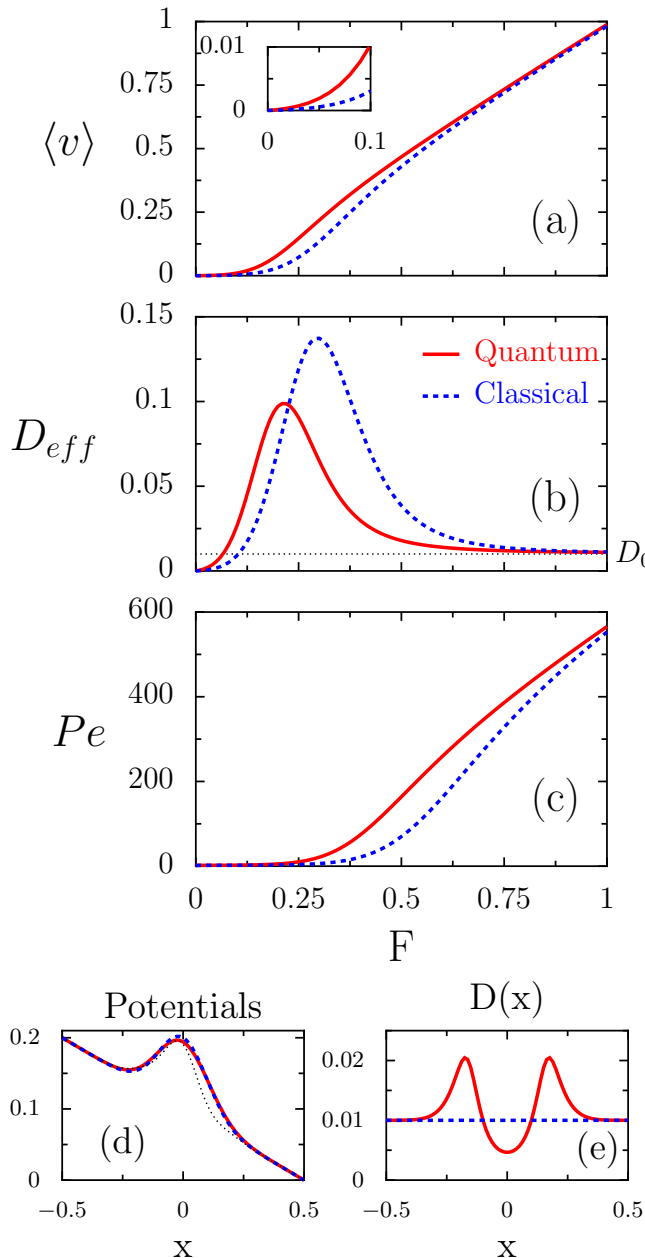
FIG. 2: Average velocity \langle v \rangle (a), effective diffusion D_{eff} (b) and Peclet number Pe (c) are drawn versus tilt F . Parameters of the potential are: \varepsilon = 100 , \Delta = 10 , which result in a barrier height of \Delta V = 0.1 in the absence of a tilt ( F = 0 ), and a critical tilt F_c \simeq 0.6 above which all barriers disappear. The rescaled inverse temperature is set to \beta = 100 , corresponding to a small quantum parameter \lambda_0 \simeq 0.00115129 . The mean velocity and Peclet number are always larger in a quantum case, even if the classical effective diffusion is smaller (as is the case for F \lesssim 0.25 ). With the panel (d) we depict the corresponding classical, U(x) , (dashed), quantum effective, U_{eff}(x) , (solid line) and thermodynamic, \psi(x) , (dotted) tilted potentials, respectively. The position-dependent diffusion coefficient is plotted in panel (e).
