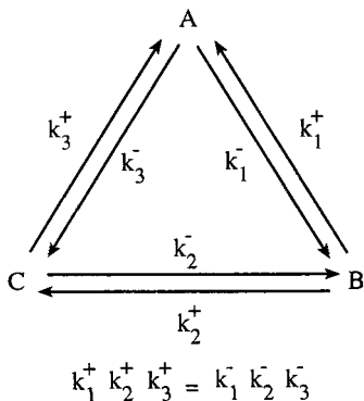
Fig. 1. Schematic representation of two fair games, and the corresponding circular chemical reaction for the second game in the spirit of Onsager. As detailed in the main text, random switching between the two fair games leads to a game that is no longer fair since the property of detailed balance is lost.
