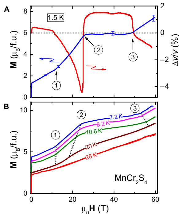
Fig. 3. Field dependence of magnetization and ultrasound velocity in \text{MnCr}_2\text{S}_4 single crystals. (A) Magnetization (left scale), in Bohr magneton per f.u. (formula unit), and relative change of the sound velocity \Delta v/v of the longitudinal acoustic mode propagating along the \langle 111 \rangle axis (right scale) at 1.5 K as a function of the external magnetic field applied along \langle 111 \rangle . Error bars mark uncertainties of calibration, which increase with increasing fields. (B) Magnetization for different temperatures between 7.2 and 28 K. For clarity, the curves at T < 28 K are shifted. Anomalies at 11, 25, and 50 T are consecutively numbered, and dotted lines indicate their temperature-dependent shifts.
