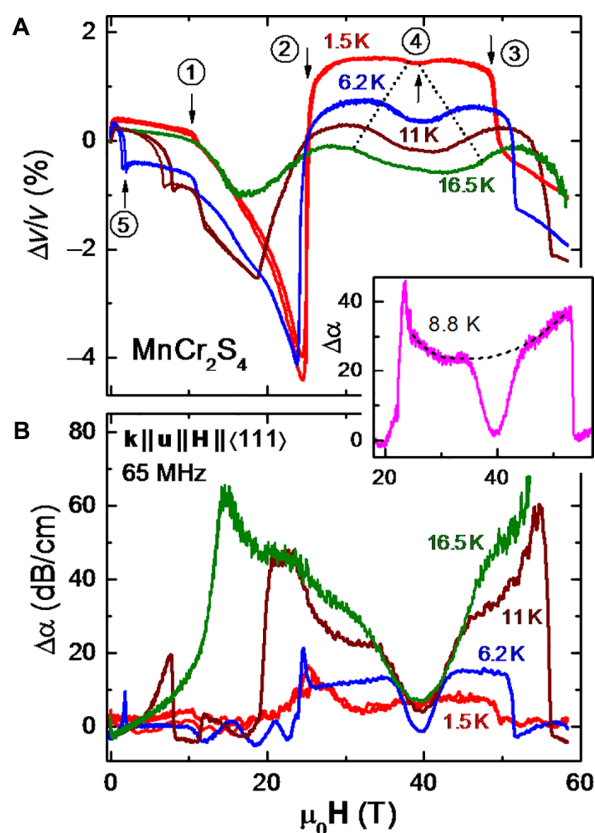
Fig. 4. Field dependence of ultrasound velocity and attenuation in single-crystalline \text{MnCr}_2\text{S}_4 . (A) Relative change of the sound velocity \Delta v/v of the longitudinal acoustic mode propagating along the \langle 111 \rangle axis versus the magnetic field at different temperatures. The external magnetic field was applied parallel to the direction of sound propagation \mathbf{k} and sound polarization \mathbf{u} . Arrows mark critical fields at the magnetostructural phase transitions. Dotted lines indicate the broadening of the phase boundaries of anomaly 4. (B) Change of the sound attenuation \Delta\alpha versus the magnetic field at different temperatures. The inset highlights the unusual damping behavior at 8.8 K and documents the suppression of damping close to 40 T. This field corresponds to an effective zero magnetic field at the manganese site. The dashed line in the inset is drawn to guide the eye.
