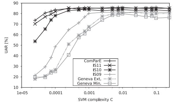
Fig. 2. Individual results (UAR [%] versus SVM complexity—all 17 values, see Section 4.3) for the EMO-DB database (categories: six basic emotions and neutral).
