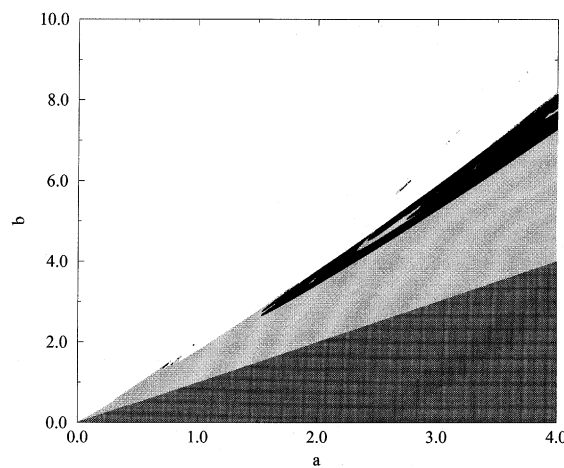
Fig. 6. Lyapunov-spectra for the jerk class \text{JD}_2 , Eq. (18), calculated for the initial values x(0) = 0.55 , \dot{x}(0) = 0.05 , \ddot{x}(0) = 0.05 . The different shades of grey classify the long-time dynamical behavior: white = divergence, dark grey = fixed point, light grey = limit cycle, black = strange attractor. To obtain a complete picture in the shown parameter region, computations have been performed up to a value for b of +10.0.
