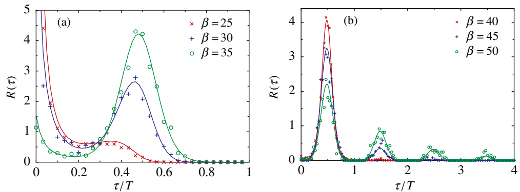
Figure 9. Residence time distributions for either of the two states are shown for \Omega = 10^{-4} and different values of the temperature. Theoretical results obtained from (equation 31) are displayed as solid lines, estimates from the simulations as symbols. In panel (a) R(\tau) is shown for higher temperatures and in panel (b) for the optimal and lower than optimal temperatures. The peak structure and its temperature dependence is in complete agreement with previous findings, see [1].
